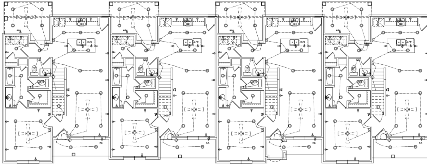
FIRST FLOOR
