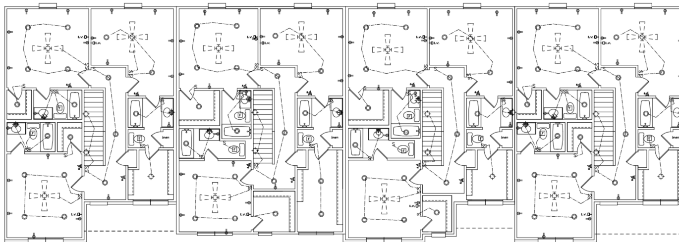
SECOND FLOOR
