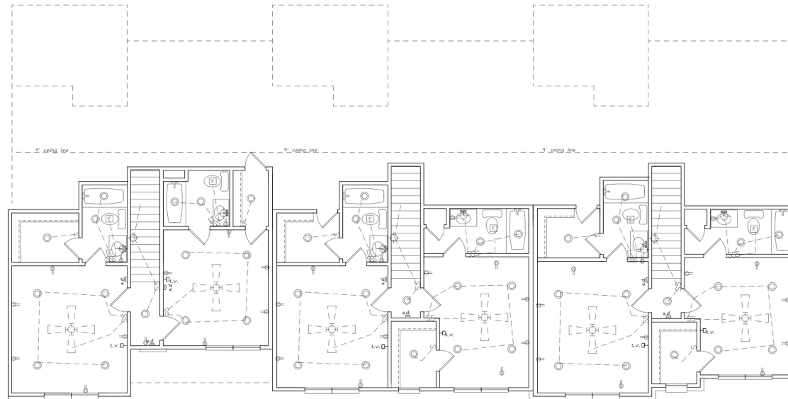
SECOND FLOOR
