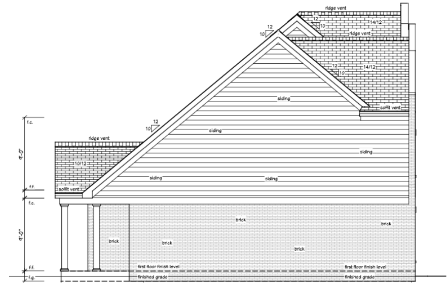
left elevation
